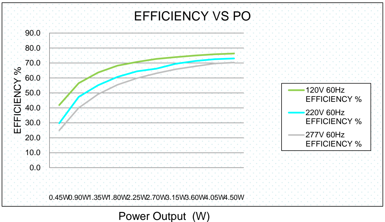
Efficiency of the driver VS Power Output (W) :
